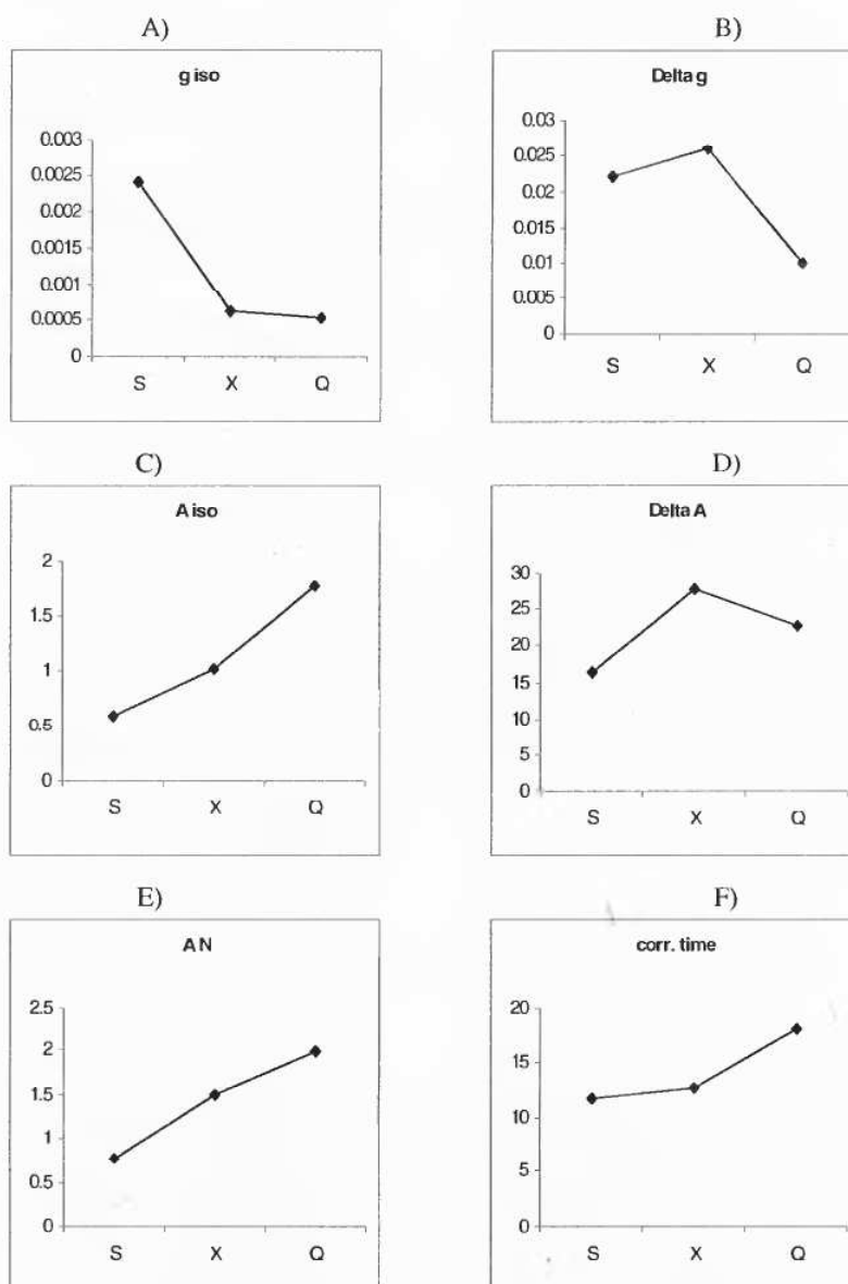
Fig. 3 Trend of the standard deviation at different frequencies for the spin-hamiltonian parameters obtained by an automatic best-fit procedure.
