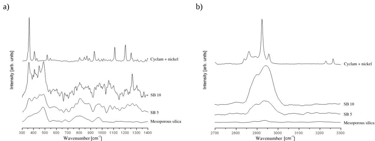
Fig. 5. Low (a) and high (b) frequency part of the resonance Raman spectra of mesoporous silica with active cyclam groups inside channels (SB5 and SB11 samples).
